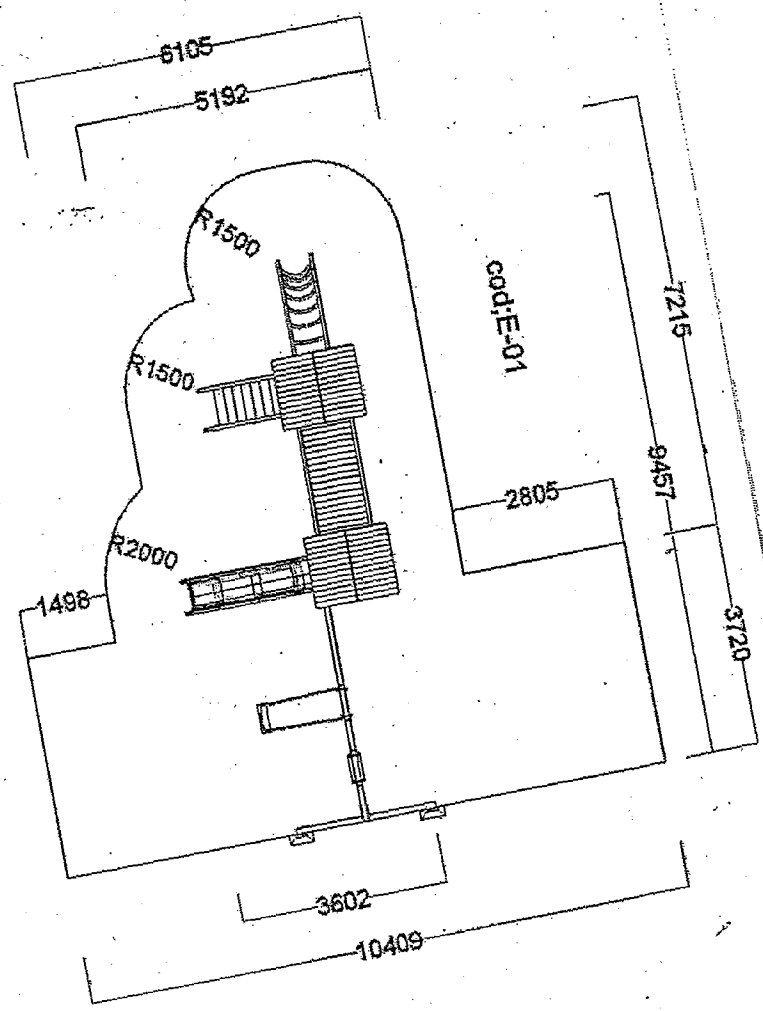
Rekvizita : "Play structure 420 kg ", Fig.23 / 1
